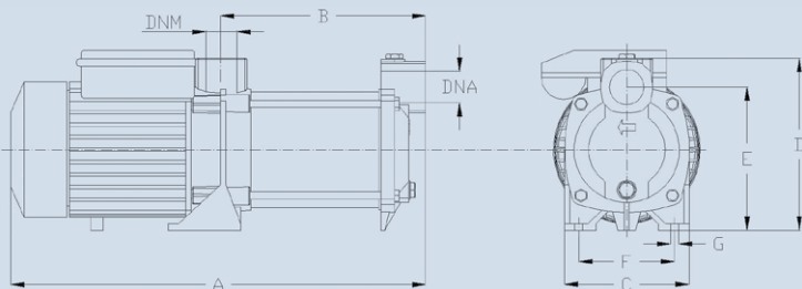
DIMENSIONI in mm. - DIMENSIONS in mm.
